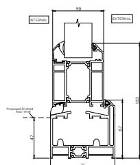
6a-6d - Threshold and Drainage Details
