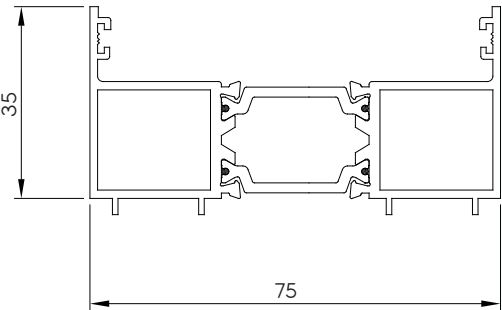
23a Bi-Fold Frame Extender Detail 23b Bi-Fold Frame Extender On Top Track
