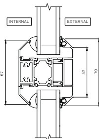
18 - Midrail Detail
