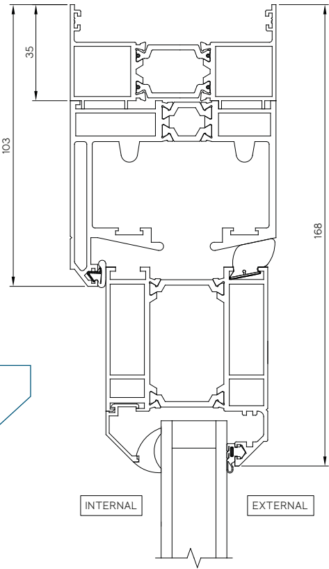
23a Bi-Fold Frame Extender Detail 23b Bi-Fold Frame Extender On Top Track
