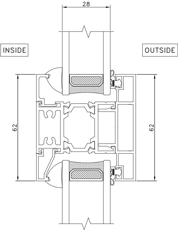
Glazing detail
