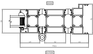
15 - Standard Mullion Detail
