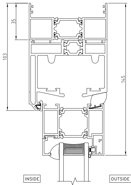
21b Bi-Fold Frame Extender With Trickle Vent Detail
