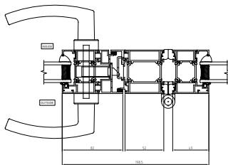
10 - Locking Slave Detail
