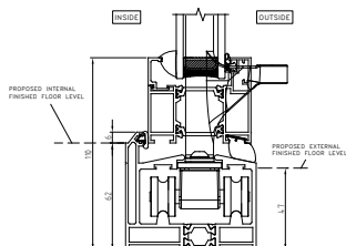
6a-6e - Threshold and Drainage Details
